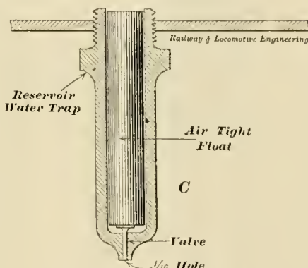
Fig. 3.—WATER TRAP FOR MAIN RESERVOIRS.
